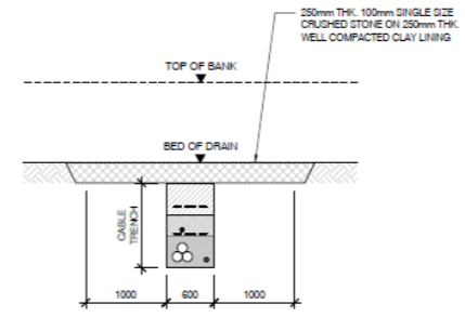
SECTION SCALE 1:50 [B]
