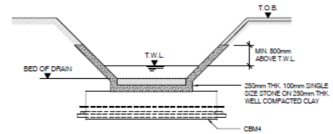
SECTION SCALE 1:100 [A]
