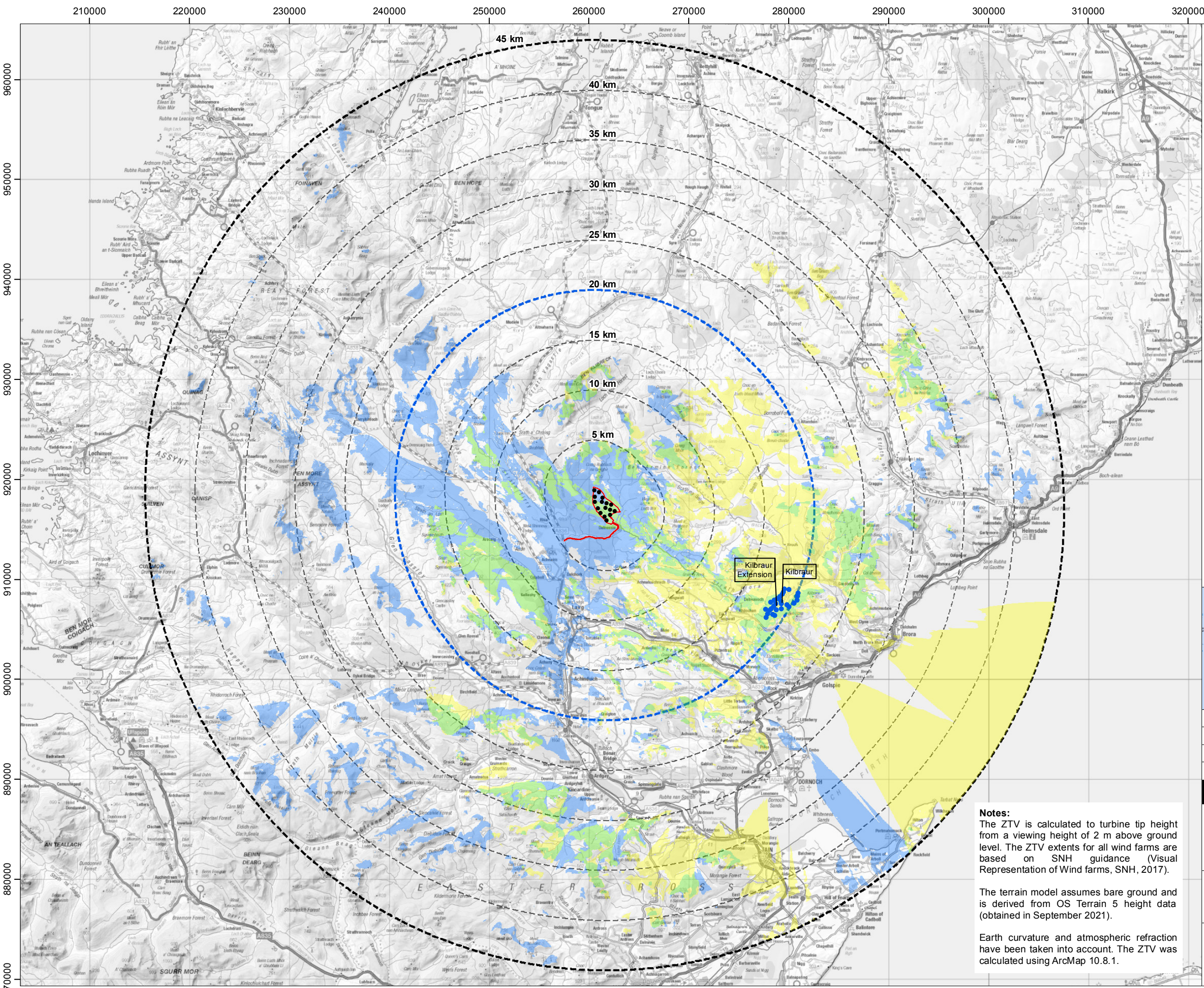
TITLE: Figure 6.1.7a: South-east Wind Farm Group Comparative ZTV (Operational and Consented)
