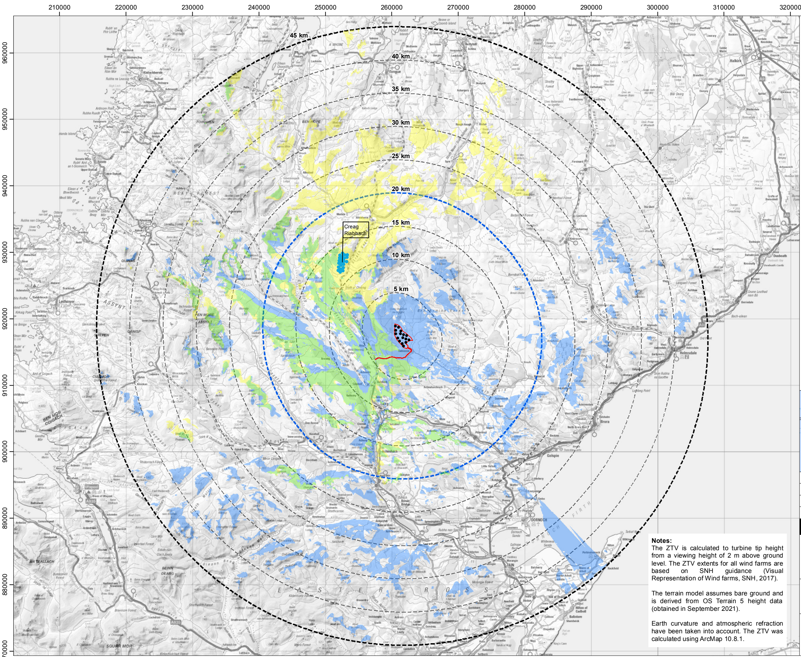
TITLE: Figure 6.1.11: Creag Riabhach (Under construction) Comparative ZTV
