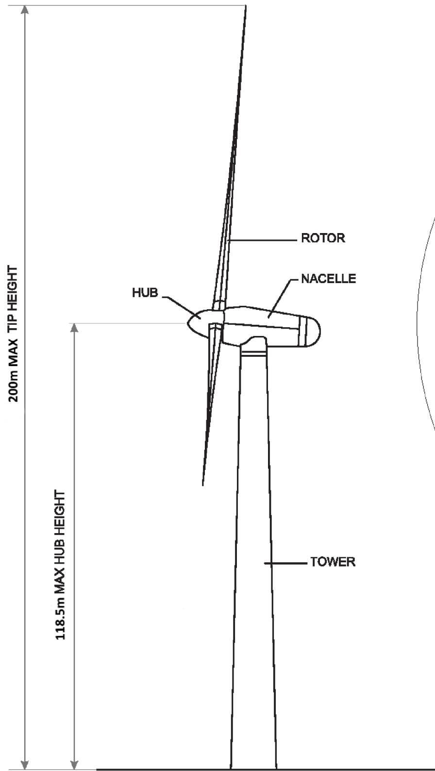
SIDE ELEVATION
